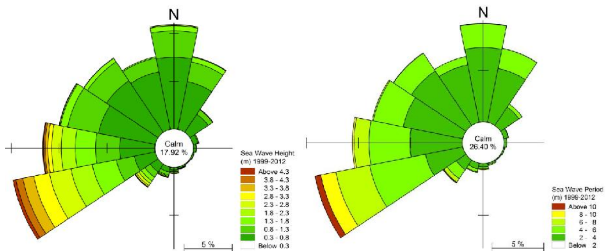
Figure 2.12 Wave rose for Sea Wave Height and Period
