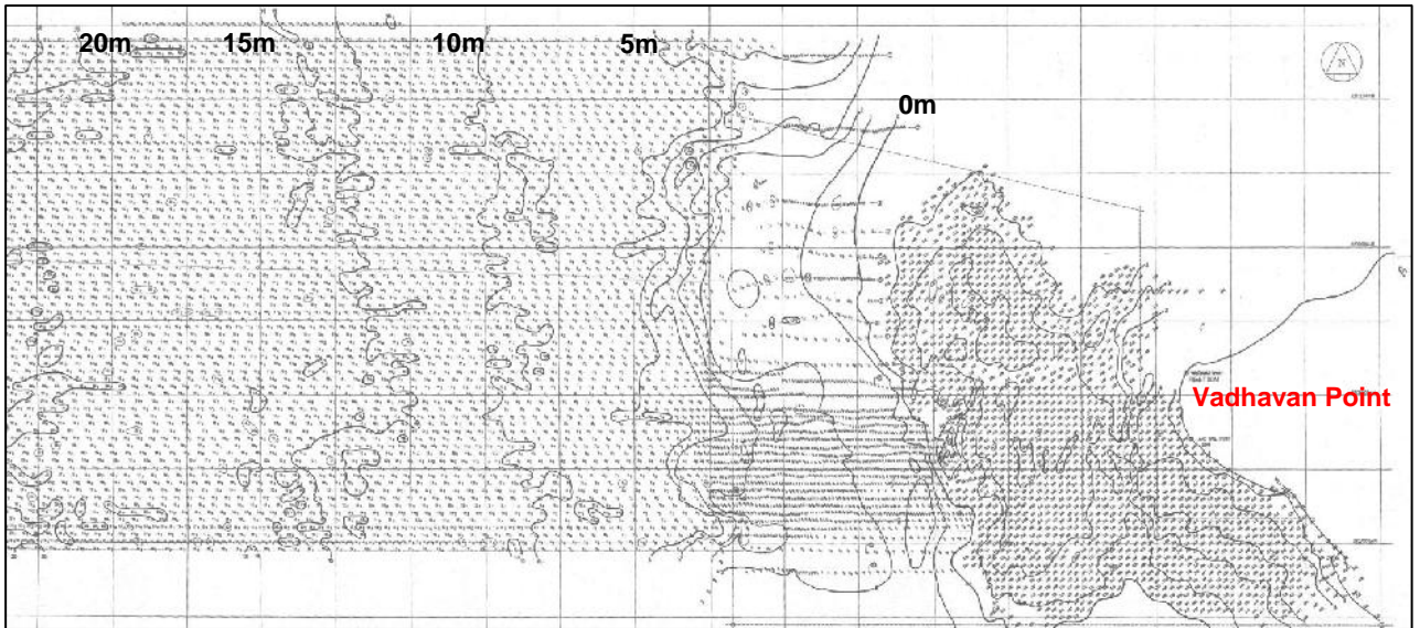
Figure 2.8 Bathymetric Survey Details at Proposed Vadhavan Port site
