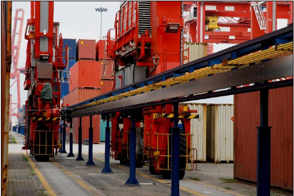
Figure 7.10 Typical Details of Electric Buss Bar Arrangement for E-RTG
