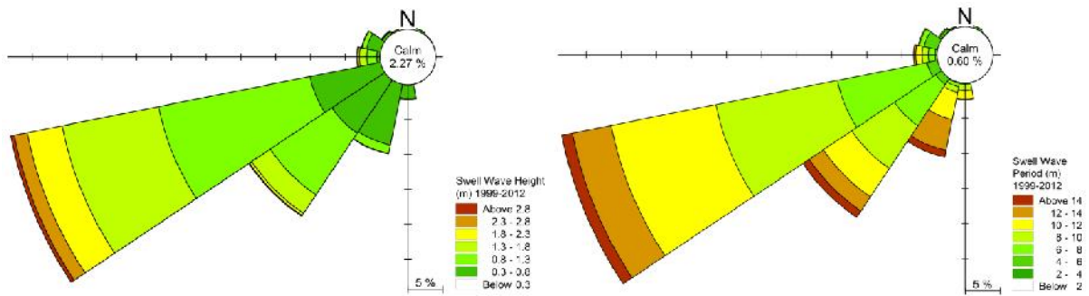
Figure 2.13 Wave rose for Swell Wave Height and Period
