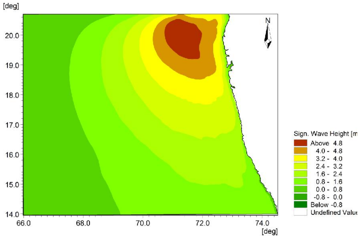
Figure 7.3 Maximum Wave height for cyclone of 1982
