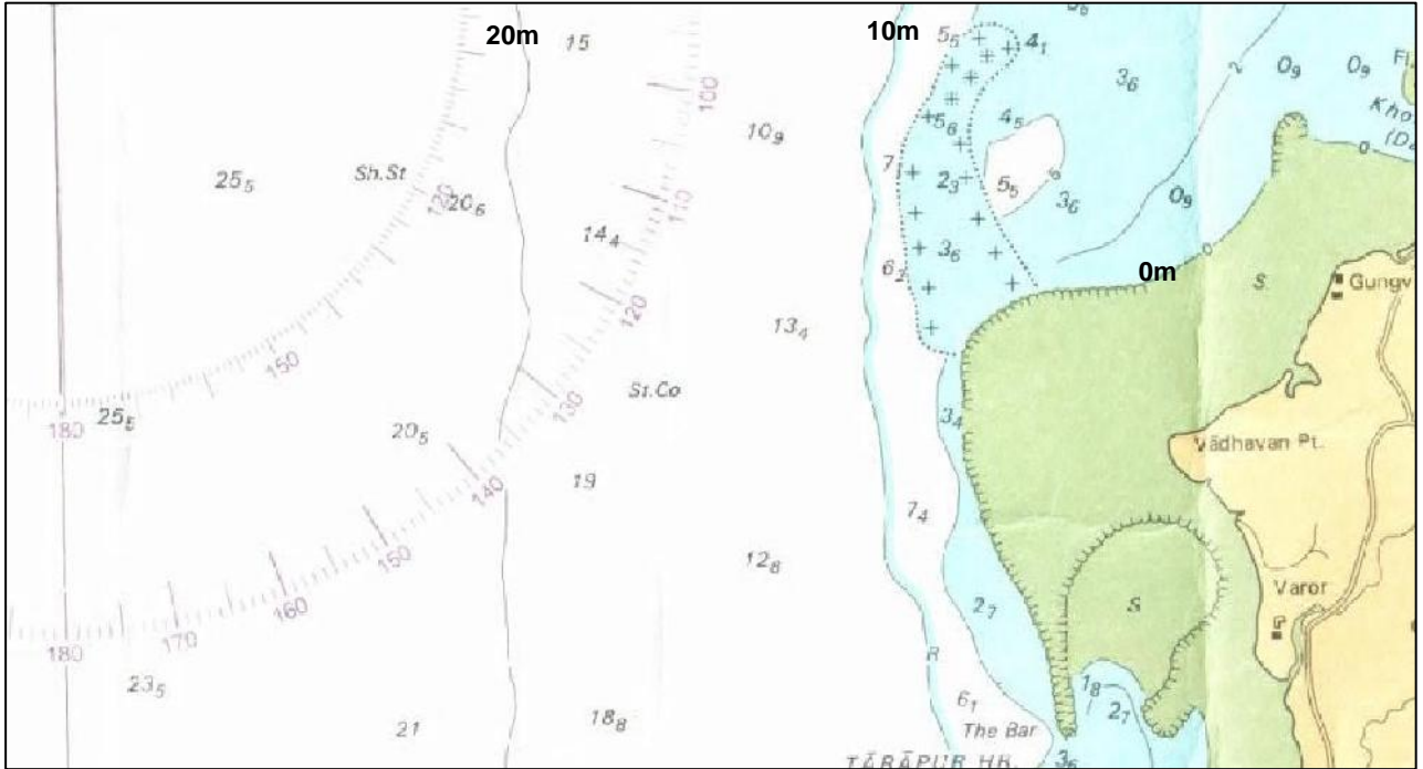
Figure 2.9 Hydrographic Chart of Vadhavan Port location
