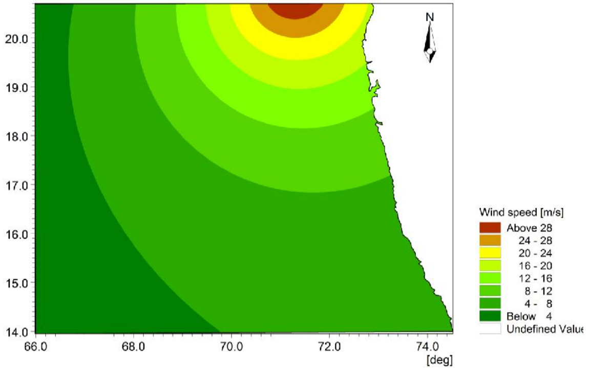
Figure 7.2 Wind Speed for cyclone of 1982
