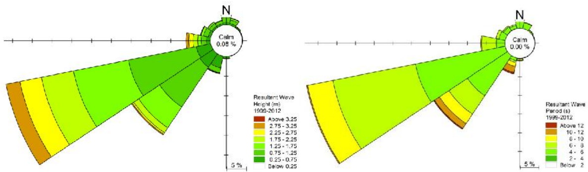
Figure 2.11 Wave rose for Resultant Wave Height and period
